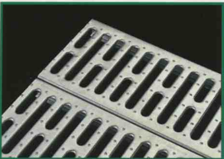
2" galvanized open steel planking
